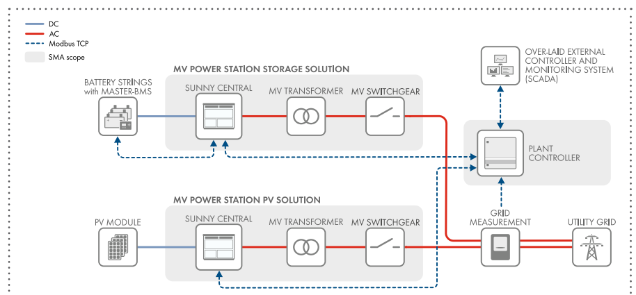
AC-coupled PV + storage system
